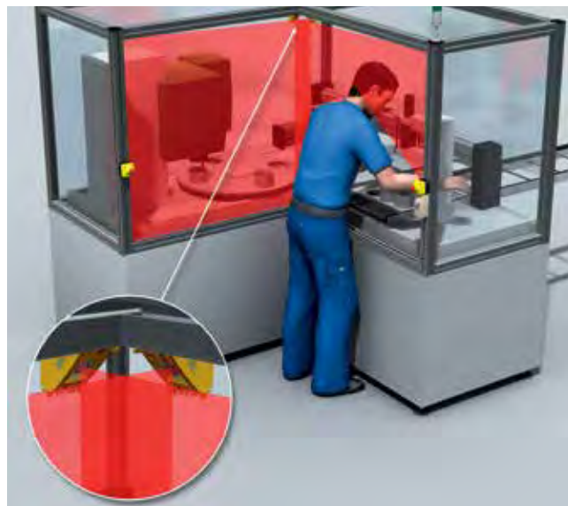
In this arrangement it is not possible to remain in the hazard zone without being detected. Therefore, a separate reset of the protective device is not necessary.
